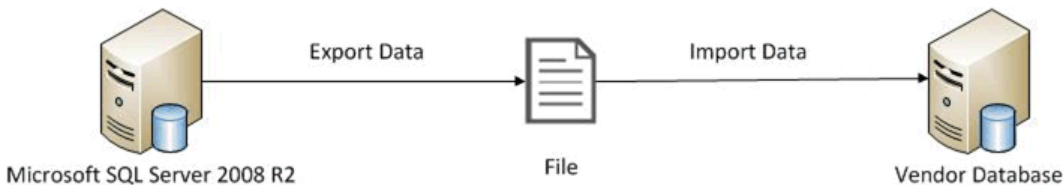
Figure 3: Import data
