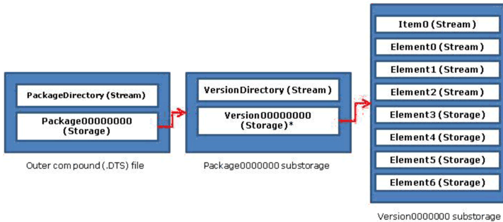
Figure 14: Structure of a DTS container file
