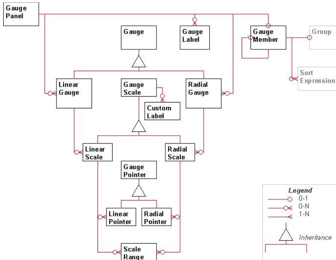
Figure 7: Gauge panel
