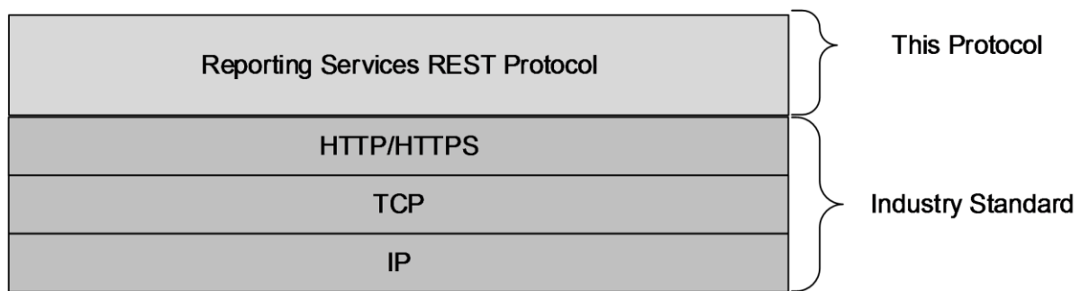
Figure 2: Protocol layering
