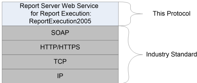
Figure 2: SOAP over HTTP or over HTTPS
