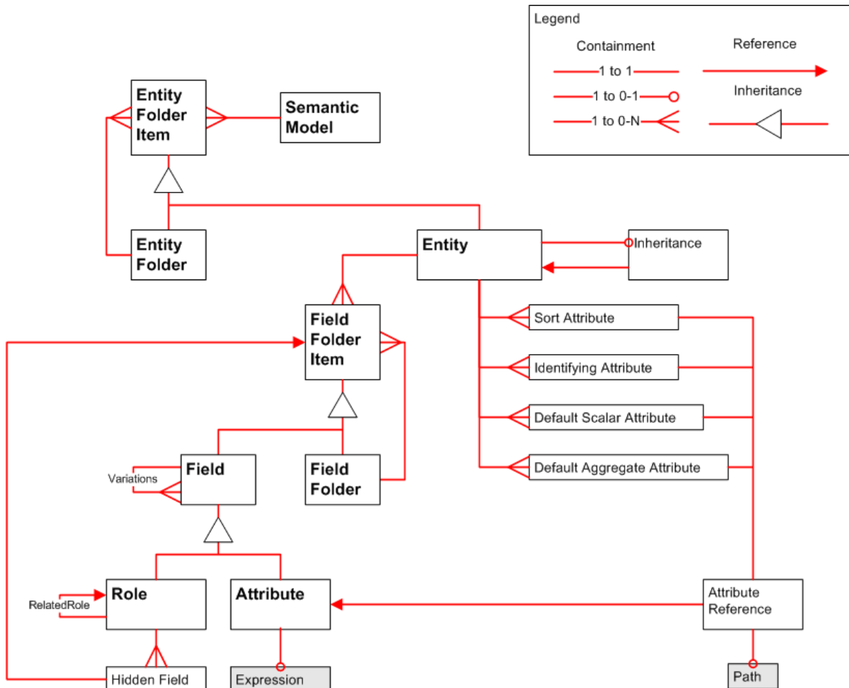
Figure 2: Semantic Objects
