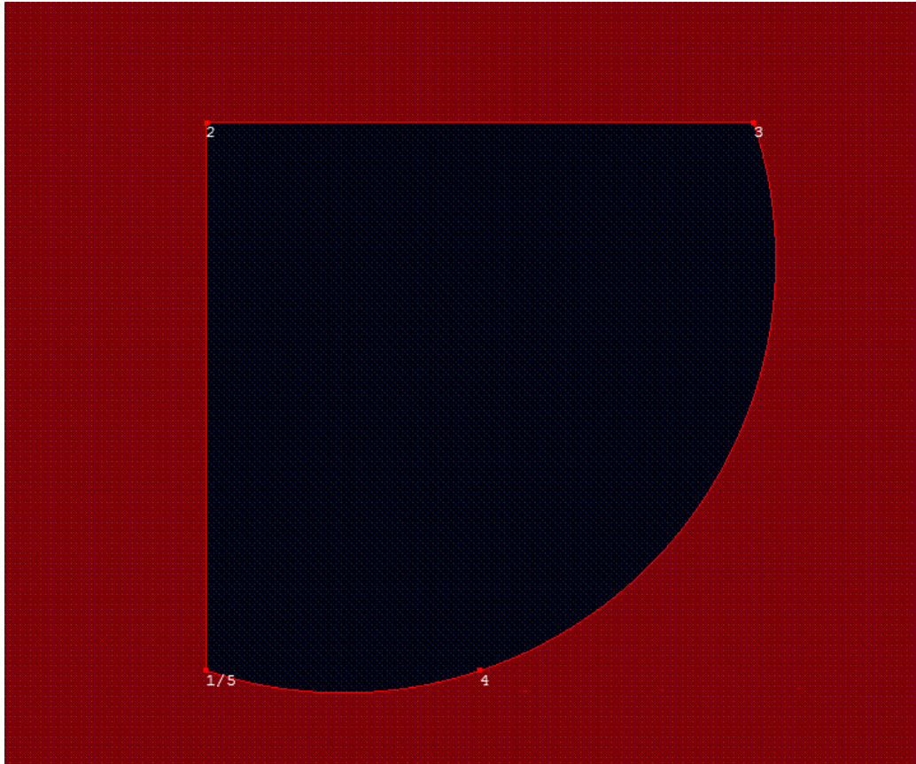
Figure 4: A curve polygon hole
