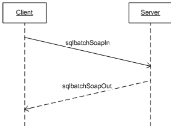
Figure 4: Single sqlbatch operation
