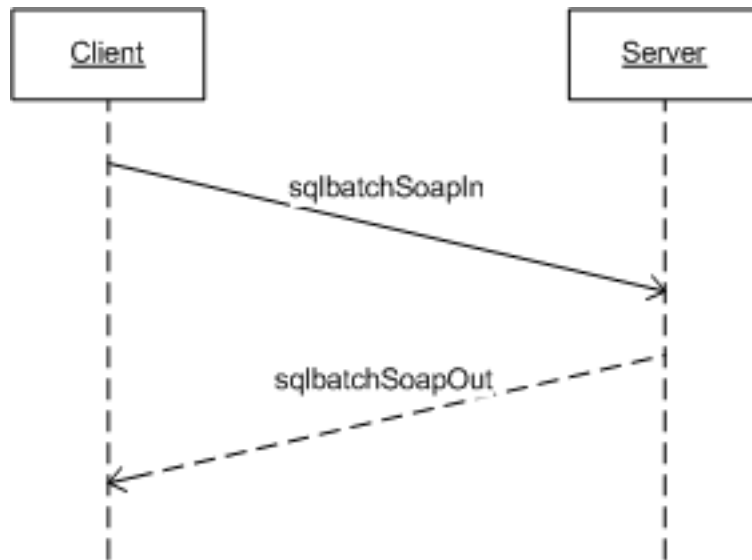
Figure 4: Single sqlbatch operation
