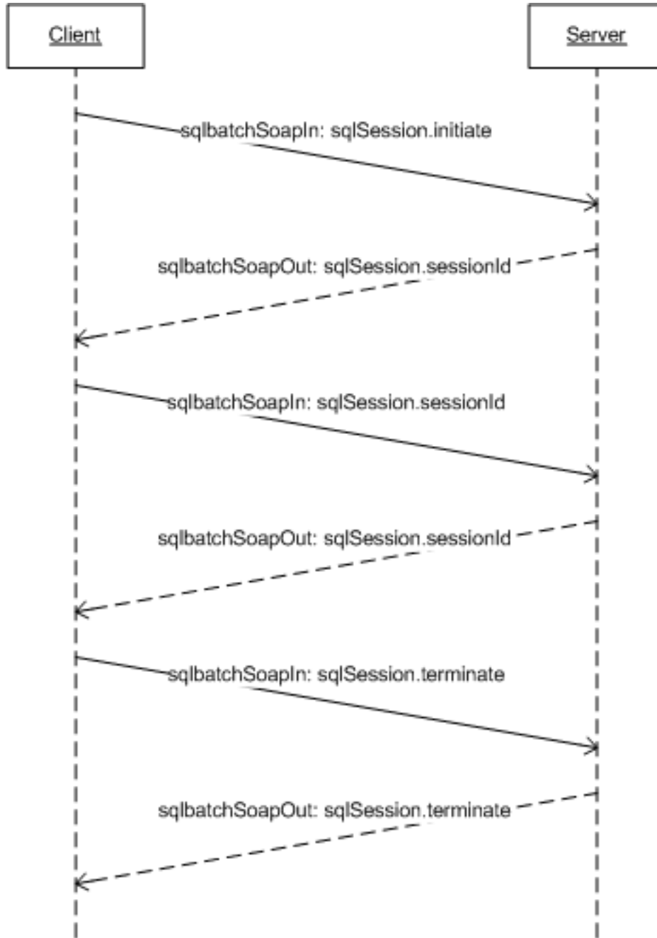
Figure 5: Session-based sqlbatch operation
