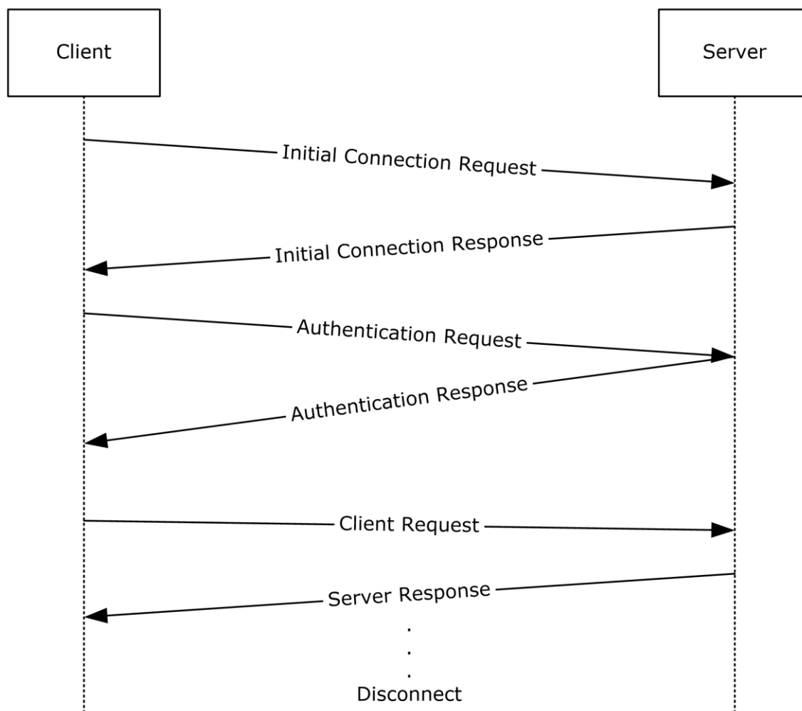
Figure 12: Client connection use case
