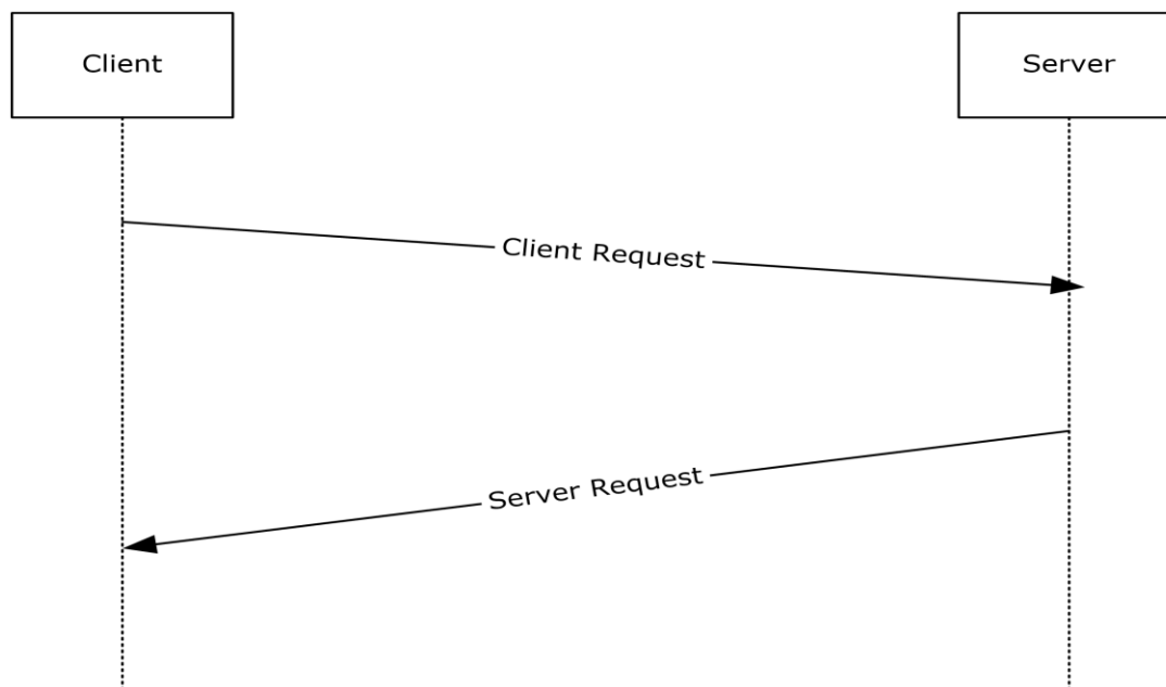
Figure 11: Named SQL Server instance resolution use case
