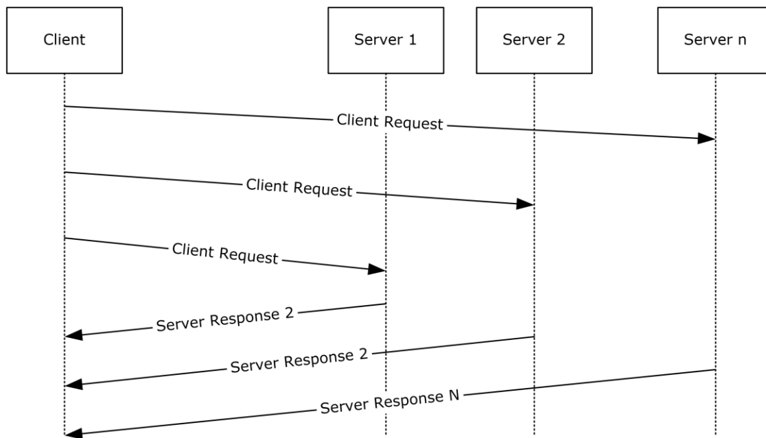
Figure 10: SQL Server instance discovery use case
